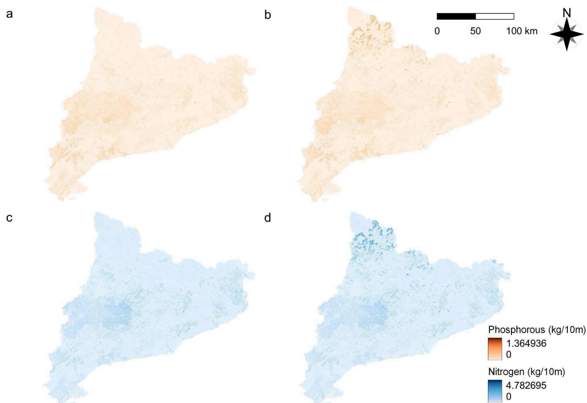
Figure 3. Nutrient Delivery Ratio model results [kg/10m] in Catalonia for (a) phosphorous surface export in a scenario with no AEP; (b) phosphorous surface export in a scenario with AEP; (c) nitrogen surface export in a scenario with no AEP; (d) nitrogen surface export in a scenario with AEP. More details on the model and calculations can be found in the nutrient model factsheet in D3.3.
